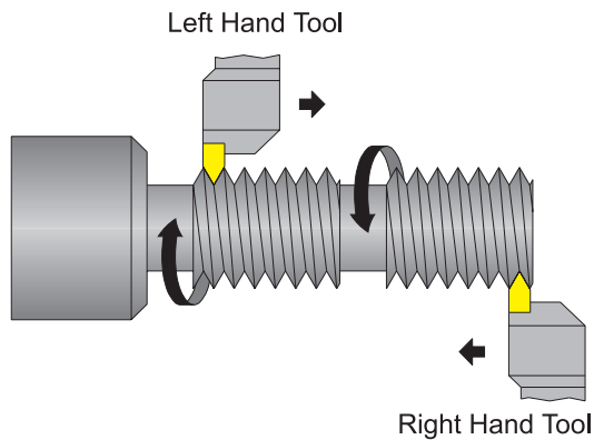
EXTERNAL RIGHT HAND THREAD
