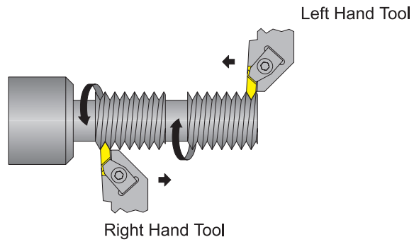
EXTERNAL LEFT HAND THREAD
