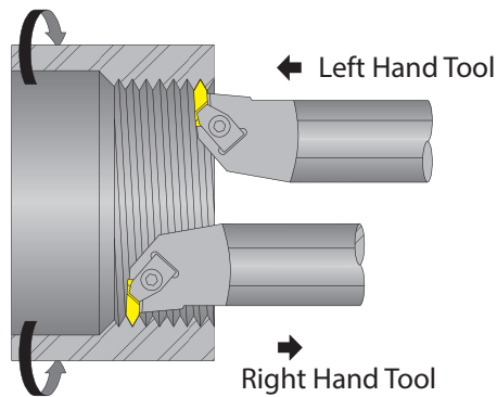
INTERNAL LEFT HAND THREAD
